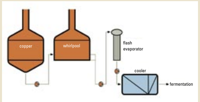
Fig. 11 Schoko wort boiling system (Schulz)
