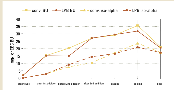
Fig. 5 Bitter substances in low-pressure boiling (according to Fig. 4) compared to conventional boiling
