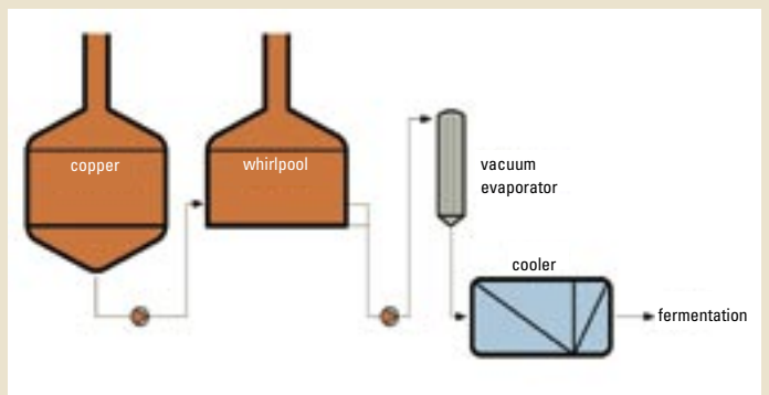
Fig. 13 Wort boiling system with flash evaporator (Ziemann)
