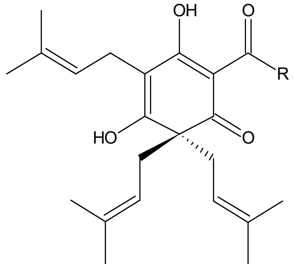
Structure of Beta acids
